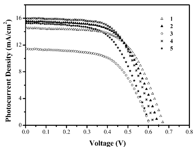
Figure 5. J – V curves of DSSCs based on the dyes.
